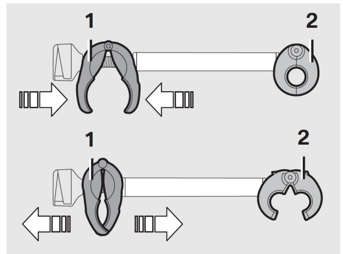
Diagram of removable retaining arms.
